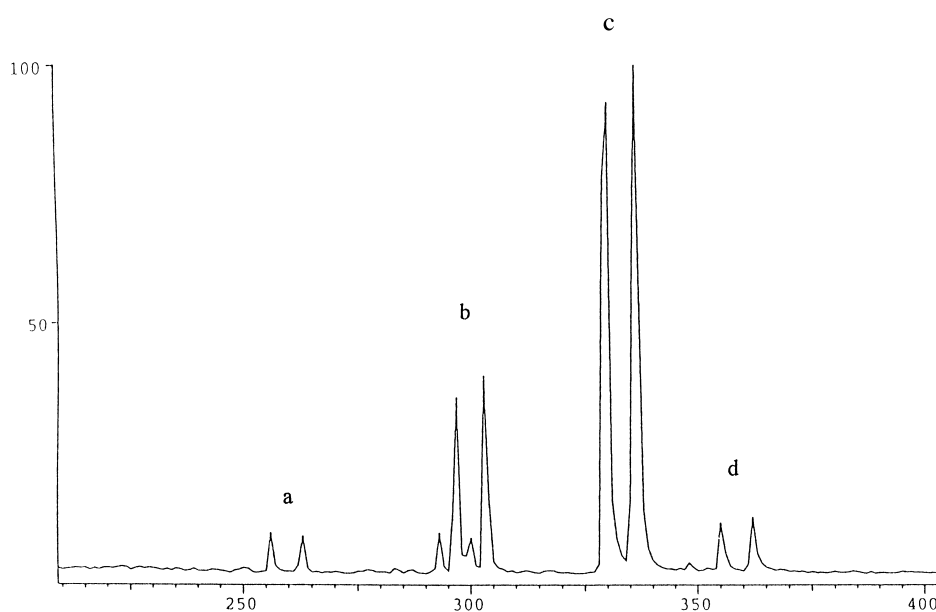
Fig. 1. Capillary gas chromatography analysis of the endogenous compounds after silylation with bis-TMS trifluoroacetamide performed on DB-5MS capillary column (15 m \times 0.25 mm). Peak identities: tetramethylsilyl ethers of the glycerol esters of (a) myristic acid; (b) palmitic acid; (c) linoleic acid; (d) arachidonic acid.
