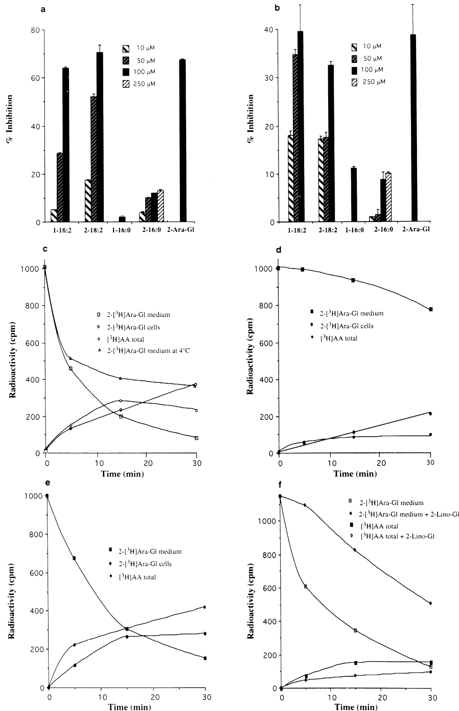
Fig. 5. Effect of monoacylglycerols on 2-Ara-Gl inactivation by RBL-2H3 and/or N18TG2 cells. (a) and (b): effect of 1-Lino-, 2-Lino-, 1-Palm-, 2-Palm- and 2-Ara-Gl on the hydrolysis of [ ^3 H]2-Ara-Gl by 10,000 \times g pellet fractions from RBL-2H3 (a) and N18TG2 (b) cells. In some cases only the effects of the doses exerting the maximal inhibition are shown. Data are means \pm S.D. of three experiments. (c–e) Clearance and hydrolysis of [ ^3 H]2-Ara-Gl by intact RBL-2H3 cells, at 37°C or 4°C (c), and in the absence (c) or presence of either 100 \mu M 2-Lino-Gl (d) or 100 \mu M 2-Palm-Gl (e) in the incubation media. (f) Clearance and hydrolysis of [ ^3 H]2-Ara-Gl by intact N18TG2 cells in the absence or presence of 100 \mu M 2-Lino-Gl. No significant inhibitory effect was obtained with 100 \mu M 2-Palm-Gl (not shown for the sake of clarity). Data in (c–f) are means of duplicates and representative of two separate experiments. Occasional differences between the radioactivity cleared from media and that found associated with cells or AA was due to non-specific binding of [ ^3 H]2-Ara-Gl to plastic, and found in the 1% bovine serum albumin washes (see Section 2).
